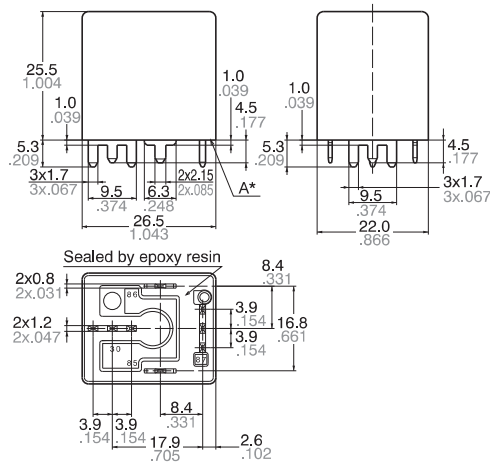
External dimensions
