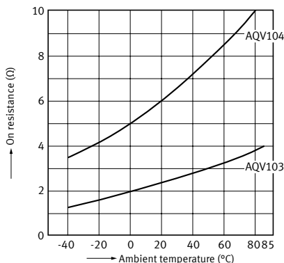
2-2. On resistance vs. ambient temperature characteristics (DC type: AQV103, AQV104)
