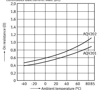
2-3. On resistance vs. ambient temperature characteristics (AC/DC type: AQV201, AQV202)
