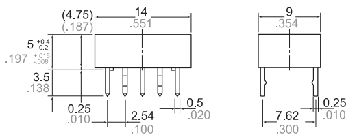
External dimensions Standard PC board terminal
